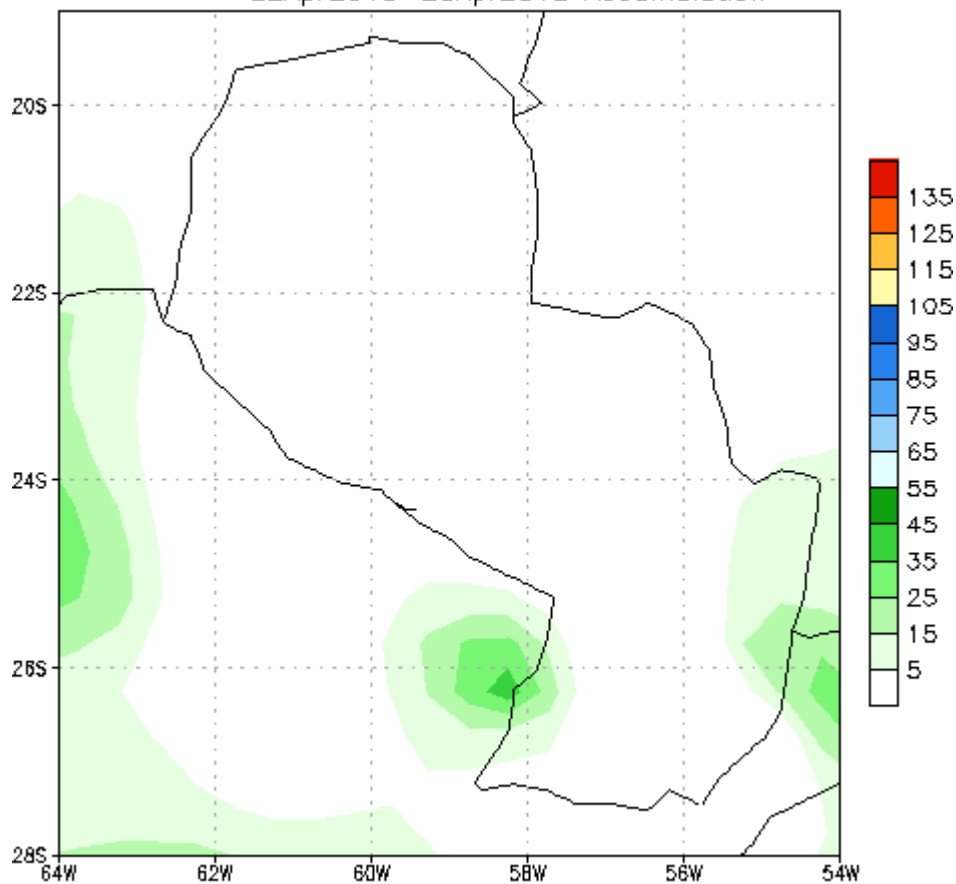
NCEP GFS Ensemble Forecast 1–7 Day Precipitation (mm) from: 22Apr2018 22Apr2018–28Apr2018 Accumulation
